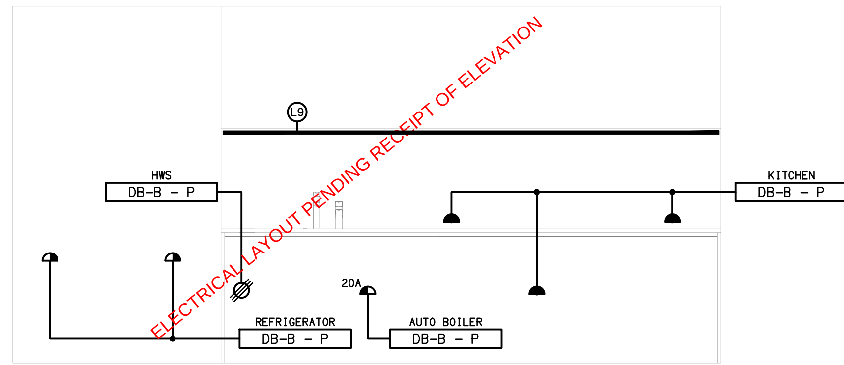
DETAIL B
